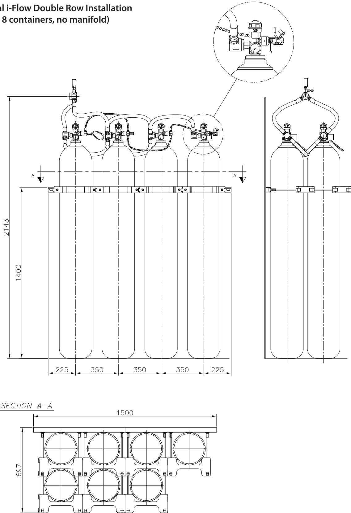
Fig. 2 iFLOW® Two Row Standard Container Bank Arrangement (no manifold)
